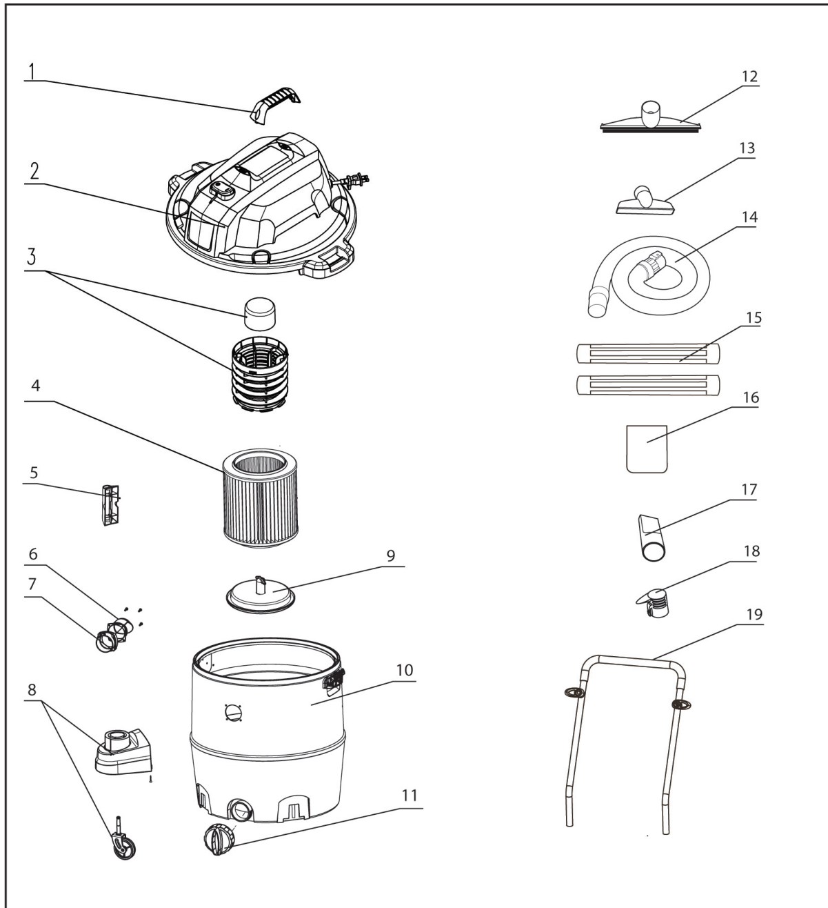
VJC1612PF 0201 Manual Parts List
